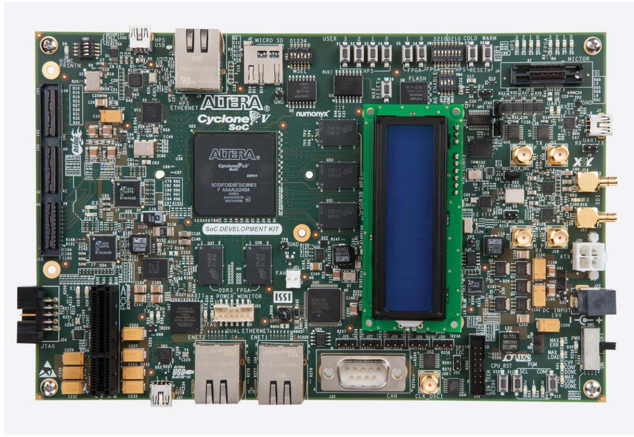
Figure 2-1. Overview of the Cyclone V SoC Development Board Features
