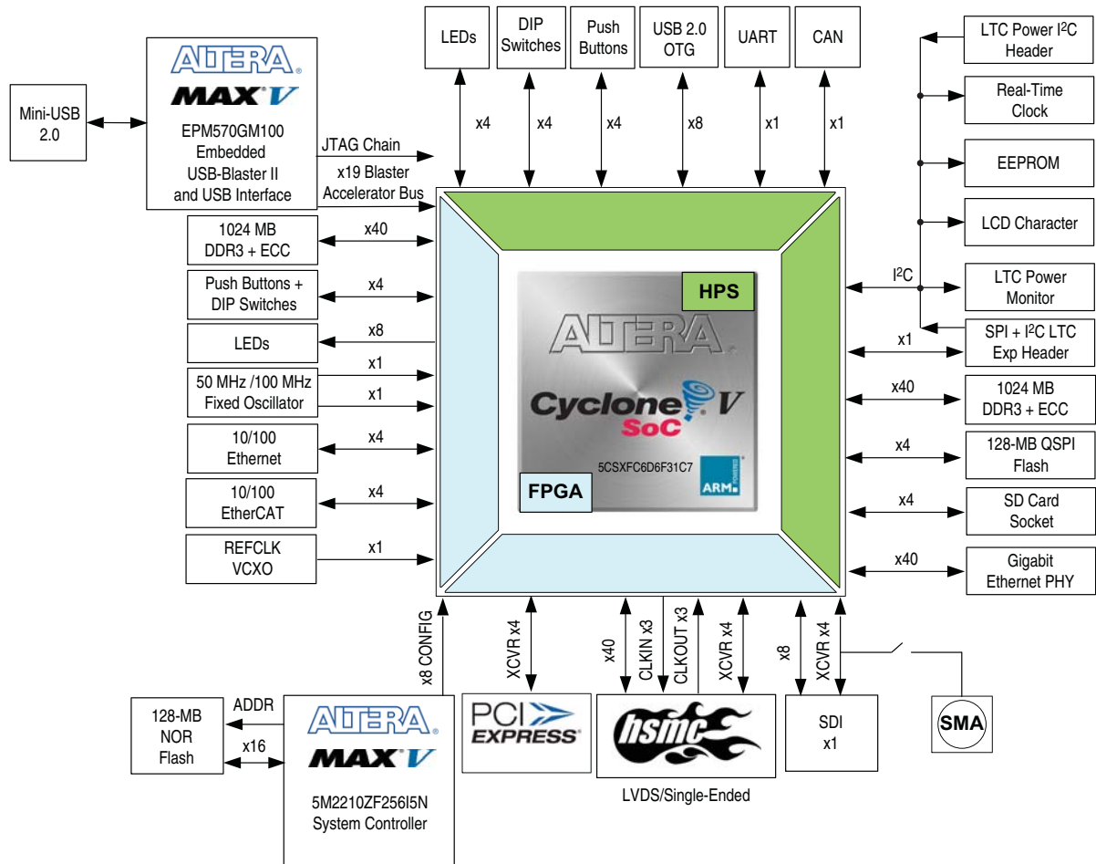
Figure 1-1. Cyclone V SoC FPGA Development Board Block Diagram
