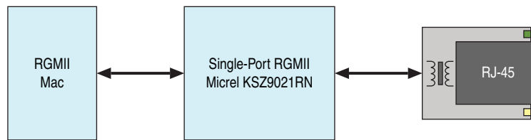
Figure 2-7. RGMII Interface between FPGA (MAC) and PHY
